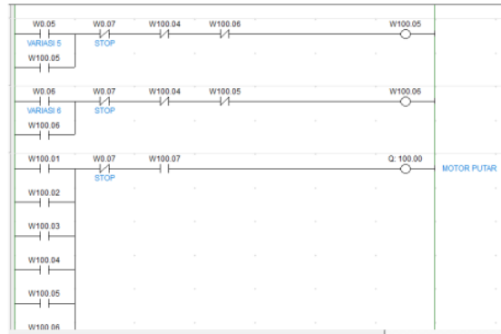
Gambar 8. Ladder Diagram 2
