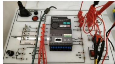
Gambar 4. Wiring Variable Speed Drive (VSD)
