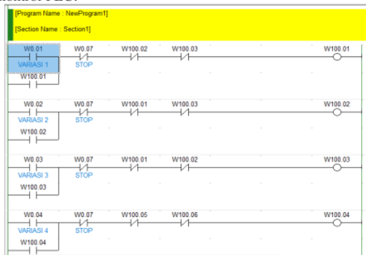
Gambar 7. Ladder Diagram 1
