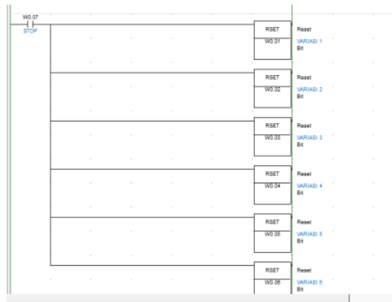
Gambar 10. Ladder Diagram 4
