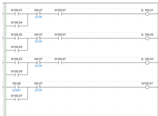
Gambar 9. Ladder Diagram 3
