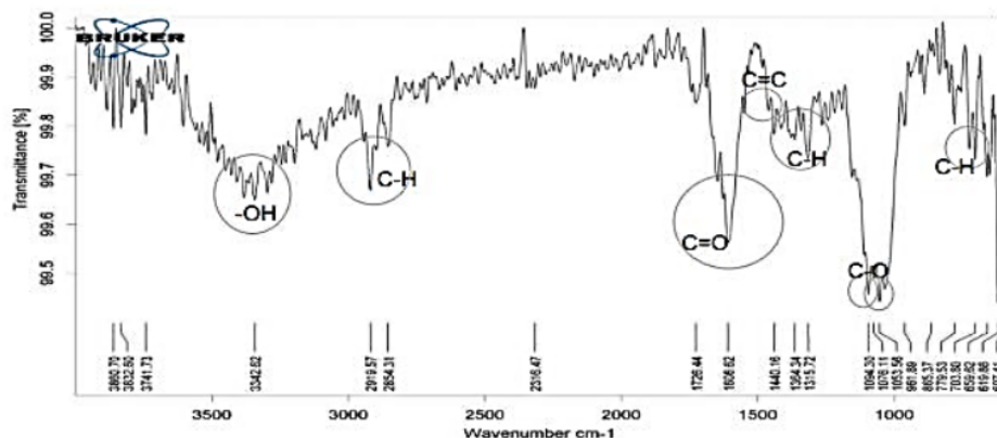
Figure 1. FT-IR Test of Paederia Foetida Leaf Powder
