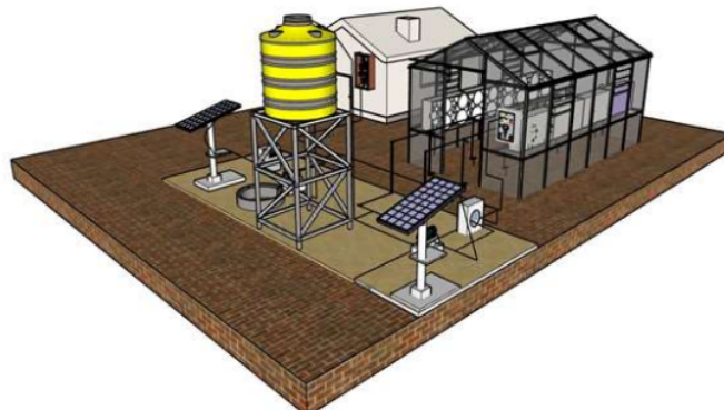
Figure 2. Fungus Cube Installation Plan
