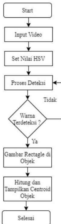
Gambar 3. Flowchart program deteksi warna
