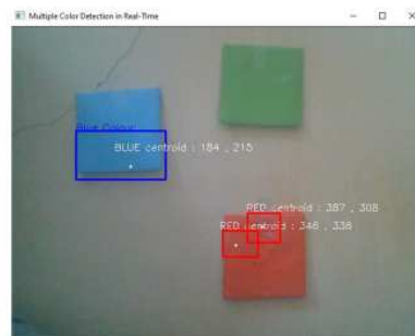
Gambar 7. Deteksi Multi-Color
