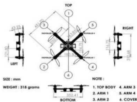
Gambar 4. Desain Quadcopter .
