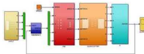
Gambar 2. Model Simulink Quadcopter .
