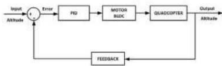
Gambar 1. Proposed Kontrol PID [9].
