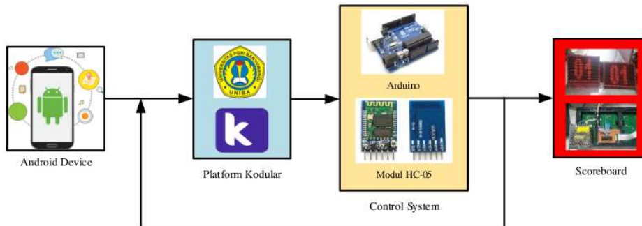
Gambar 2. Desain Sistem Kontrol Scoreboard
