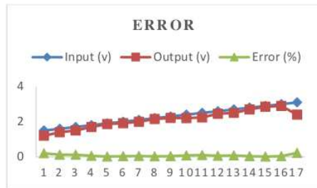
Gambar 4. Error Transmisi Scoreboard
