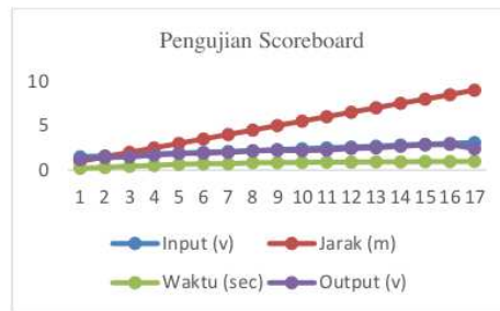
Gambar 3. Pengujian Scoreboard
